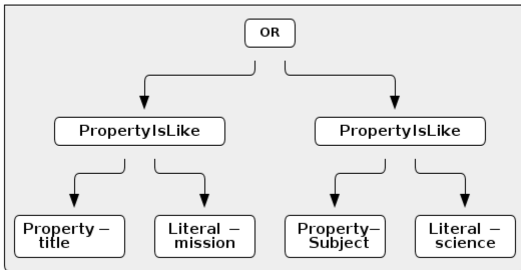
Parsing Filters XQuery
