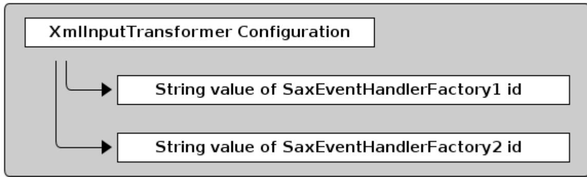
XmlInputTransformer Configuration
