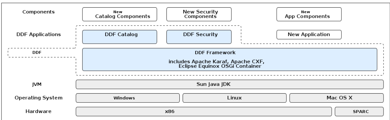
Architecture Diagram
